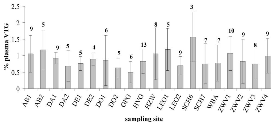
Fig. 3. Relative plasma vitellogenin (VTG) content of the eels sampled at different locations in Flanders, represented as mean \pm standard deviation. The number of fish is given for each sampling site.
