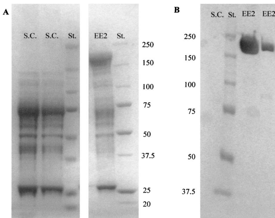
Fig. 2. (A) A typical gel after protein electrophoresis of plasma of ethinylestradiol-exposed eel (EE2) and solvent control eel (S.C.) and (B) a typical Western blot gel. Values indicate the molecular weight of the protein standard (St.), given in kilodaltons.
