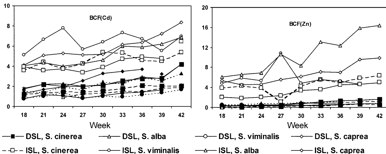
Fig. 3 Evolution of the bioconcentration factor (BCF) during a growing season for willows on dredged sediment landfills (black symbols) and infrastructure spoil landfills (open symbols) for S. cinerea (squares), S. alba (triangles), S. viminalis (circles) and S. caprea (diamonds).
